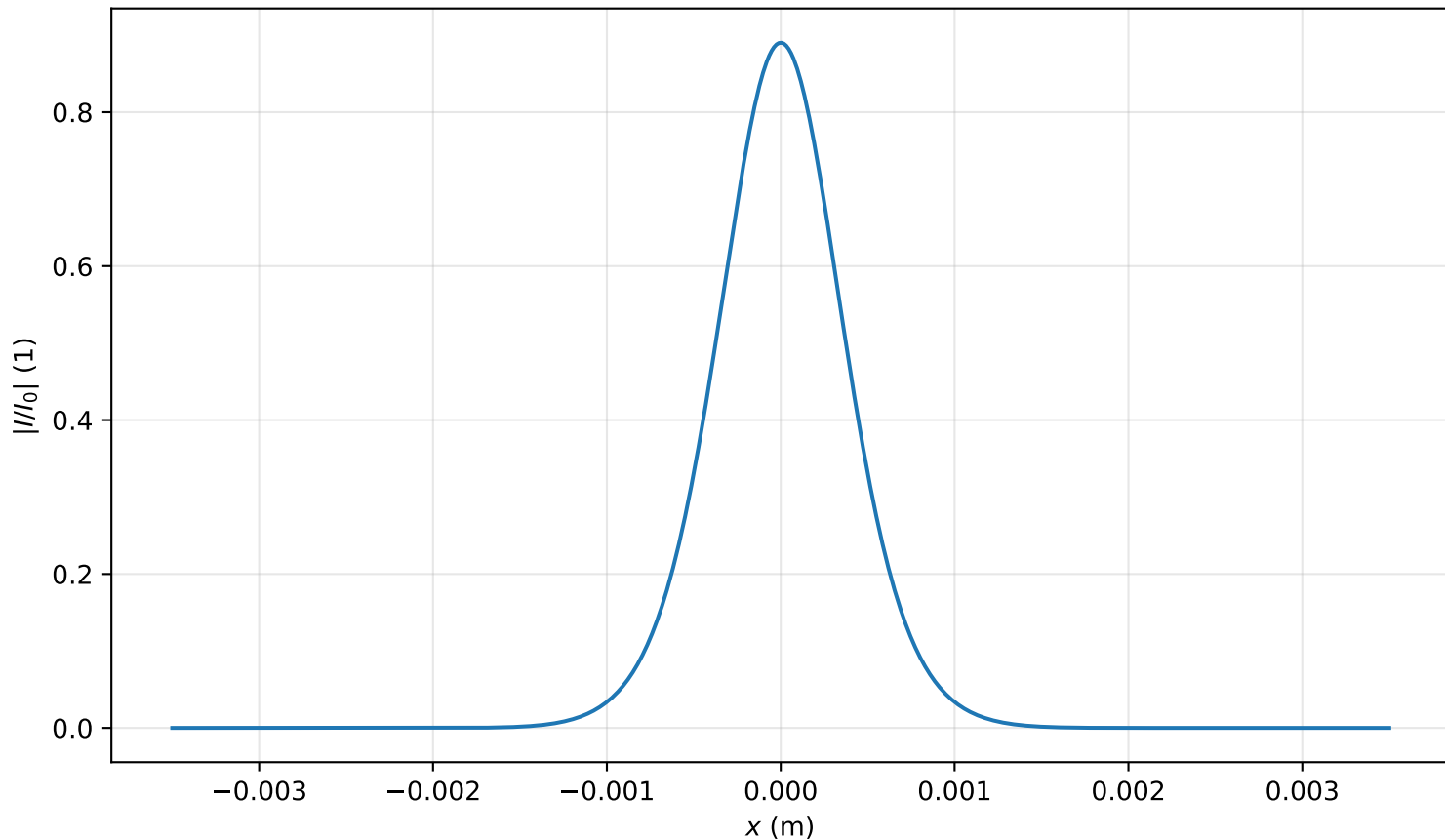
Intensity profile I(x, y = 0, z = 1.433m)/I_0 , P_{in}=0.4P_{cr} , artificial time
